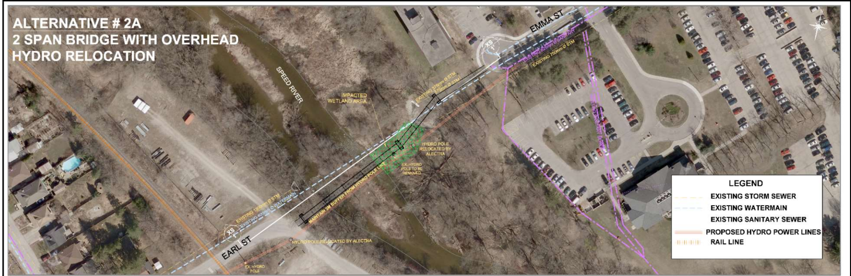
Figure 4-3 Alternative 2a: Double Span Steel Truss Bridge Through Hydro Corridor (Overhead Hydro Relocation)
